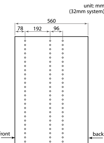
Hole pattern of side panel
