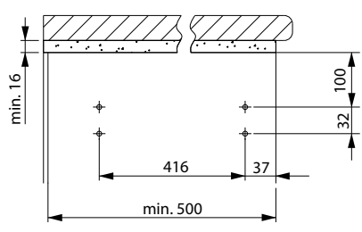
Assembly instruction (side view)
