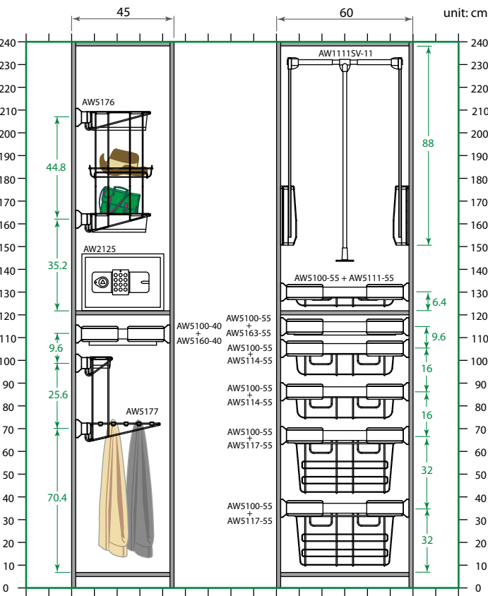
H type closet cabinet
